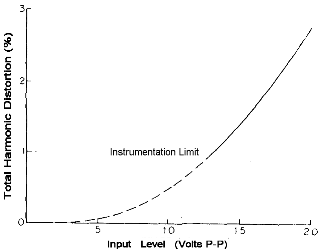
Figure 5. SAD-1024 Distortion vs. Input Level.
