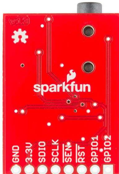
Underside of breakout board showing pin labels
