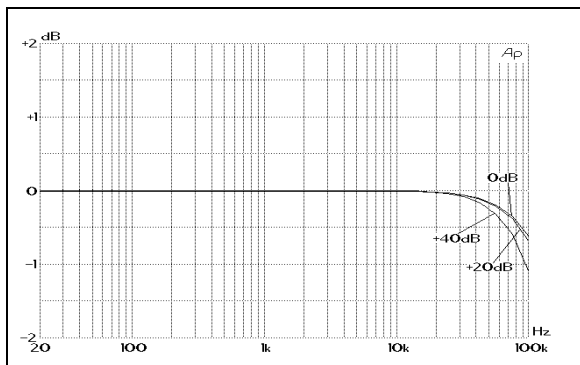
Figure 3. 2181 Series Frequency Response Vs. Gain
