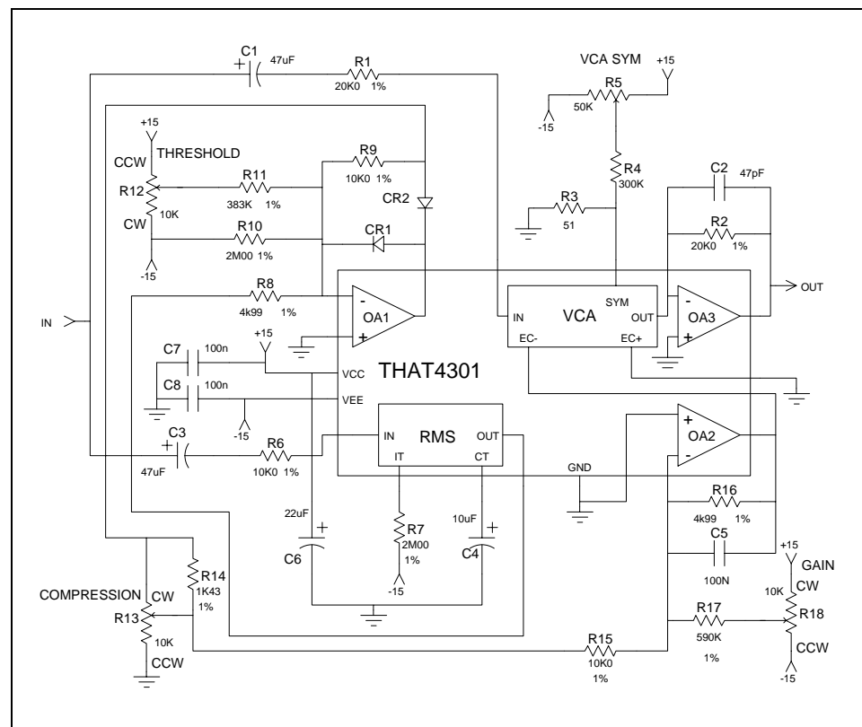
Figure 14. Typical Compressor/Limiter Application Circuit
