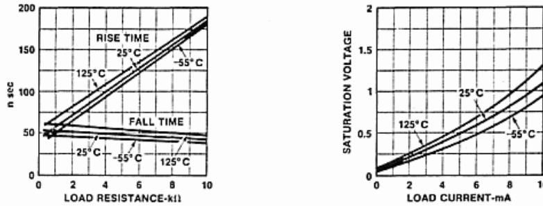
Performance of the Square-Wave Output
