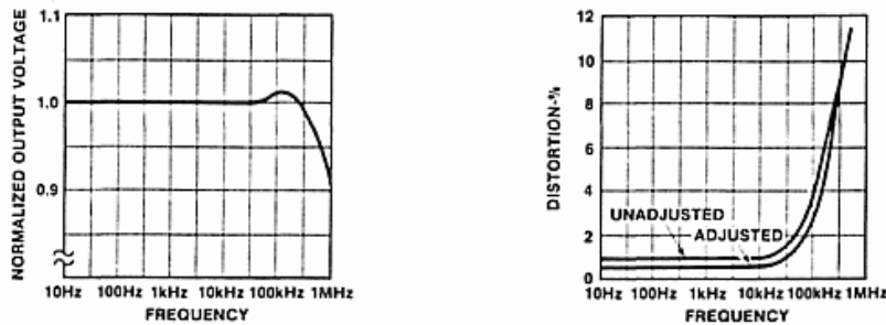
Performance of Sine-Wave Output
