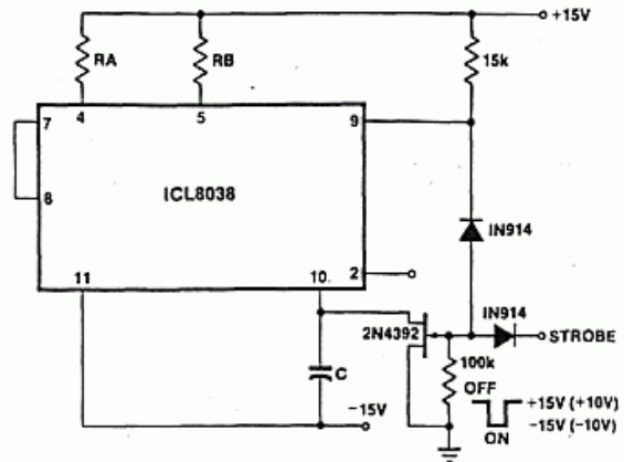
Figure 5: Strobe-Tone Burst Generator. With a dual supply voltage the external capacitor on Pin 10 can be shorted to ground to halt the 8038 oscillation. Figure 5 shows a FET switch, diode ANDED with an input strobe signal to allow the output to always start on the same slope.
