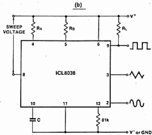
Figure 3: Connections for Frequency Modulation (a) and Sweep (b)
