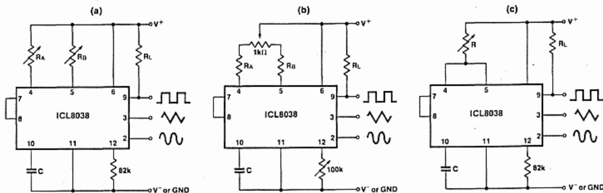
Figure 1: Possible Connections for the External Timing Resistors.
