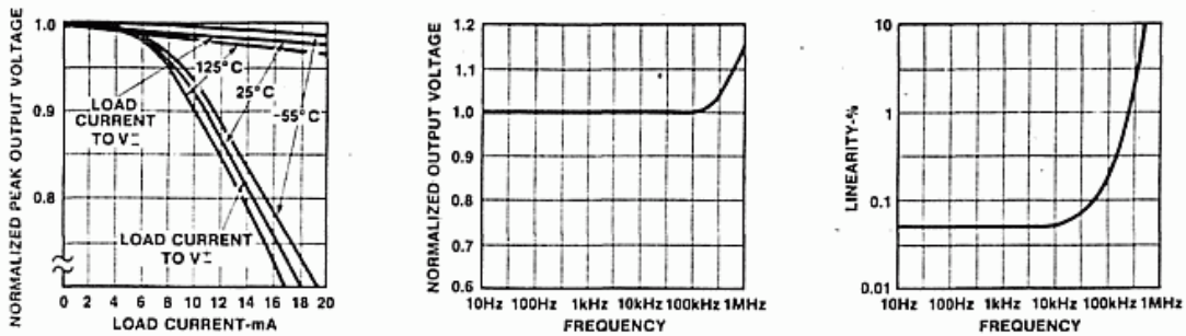
Performance of Triangle-Wave Output
