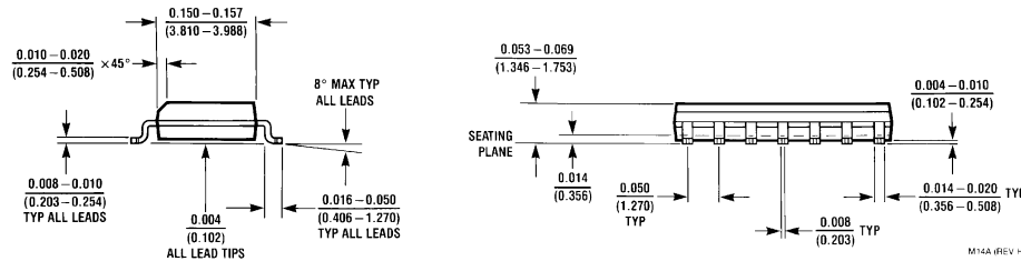
14-Pin Small Outline Package Order Number LM6144AIM or LM6144BIM NS Package Number M14A
