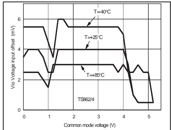
V_{IO} versus V_{ICM} and temperature at V_{CC} = 10V
