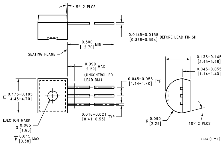
3-Lead TO-92 Plastic Package (Z) NS Package Number Z03A
