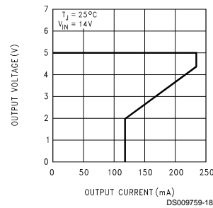
Current Limit
